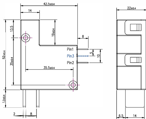
单线圈 SINGLE COIL
